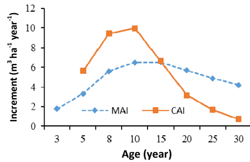
Figure 2. Trend over time (in years) for MAI and CAI of agarwood trees in Model I
