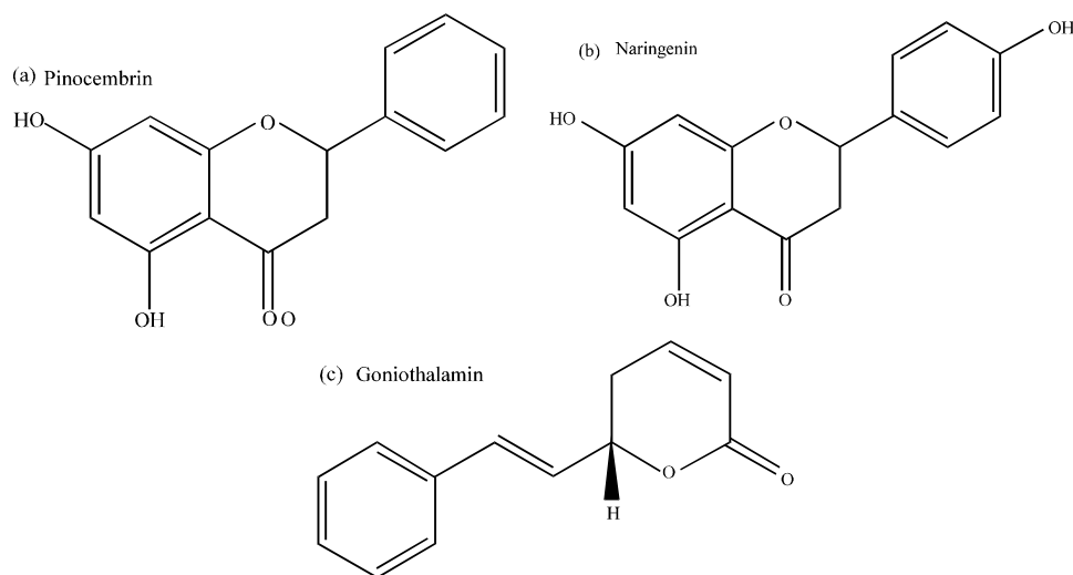
Fig. 2: Structure of compounds in Goniothalamus species
