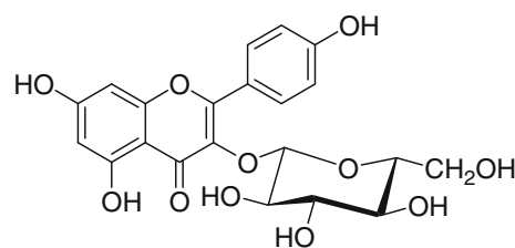
Fig. 1 Structure of compound 1
